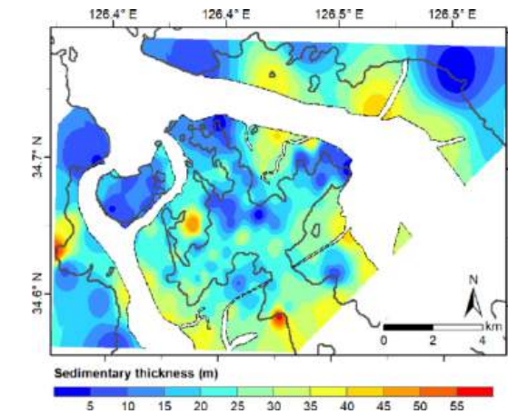
Distribution of depths to bedrock across the study area, calculated from HVSR-derived resonance frequencies and MASW shear-wave velocities.
