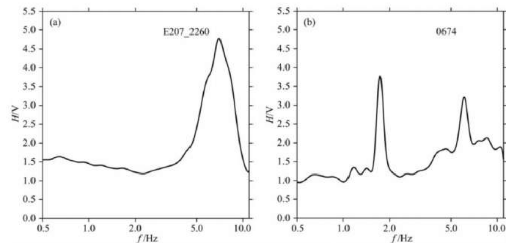
(a) Example of a single-peak HVSr curve for station E207_2260. (b) Example of a double-peak HVSr curve for station 0674.
