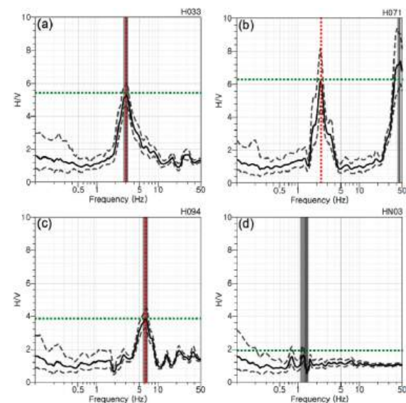
(a) HVSR curve with a single peak at a medium frequency. (b) HVSR curve with multiple peaks. (c) HVSR curve with a single peak at a higher frequency. (d) HVSR curve with no peak.
